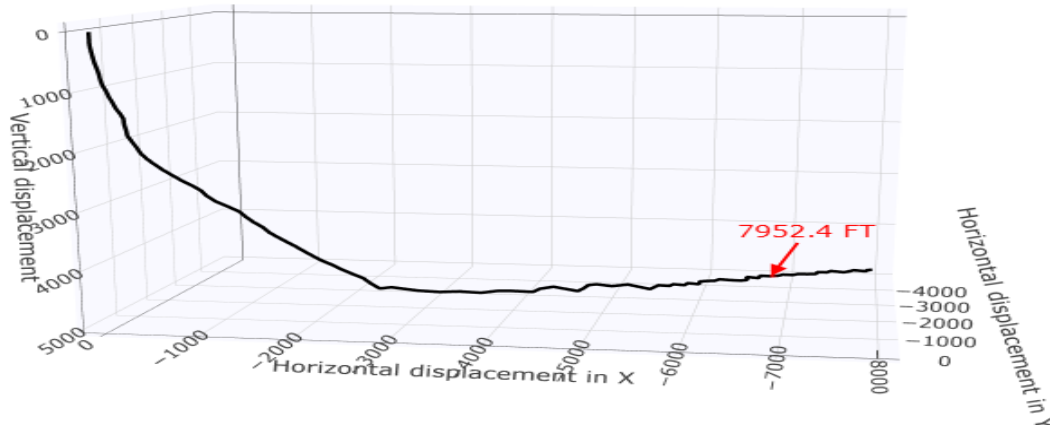
Fig.4.47: 3D-Plot for Well B sing Combined Test Method.
