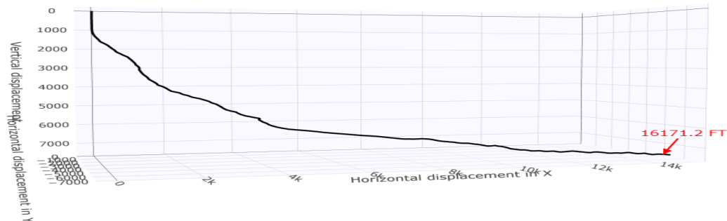
Fig12: Stuck Depth Identification on 3 D plot for Well B
