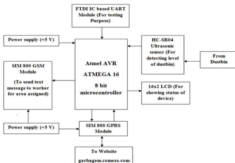
Fig 1: Block diagram of IOT based garbage management system
