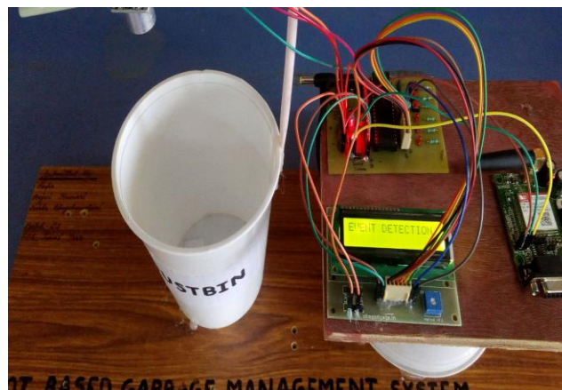
Fig 4: Event detection mode
