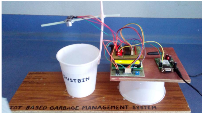
Fig 3: Complete setup of IOT based garbage management
