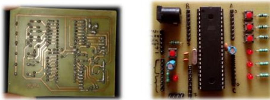
Fig 2: General purpose ATMega 16 board
