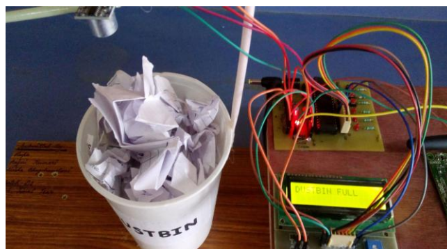
Fig 5: Dustbin full mode
