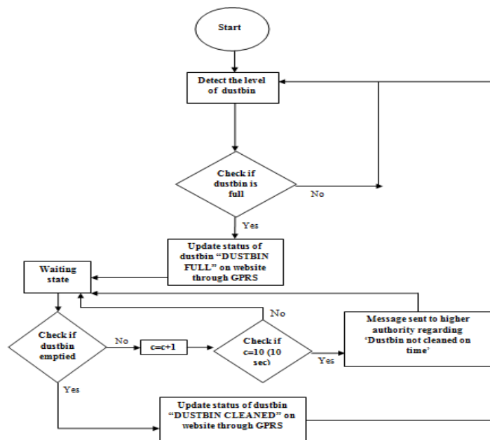
Fig 2: Flow chart of IOT based garbage management system
