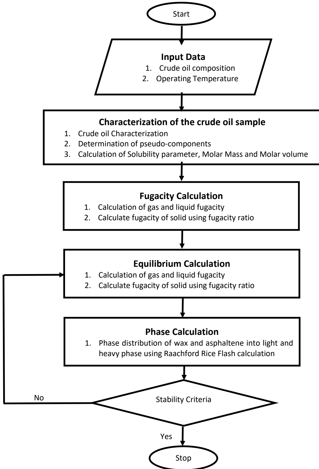
Figure 3 Modeling algorithm of the regular solution model
