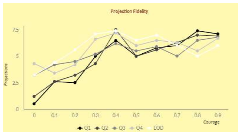
Projection Fidelity
