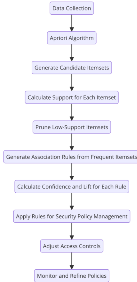
Fig 3.5a. Association Rule Mining Diagram
