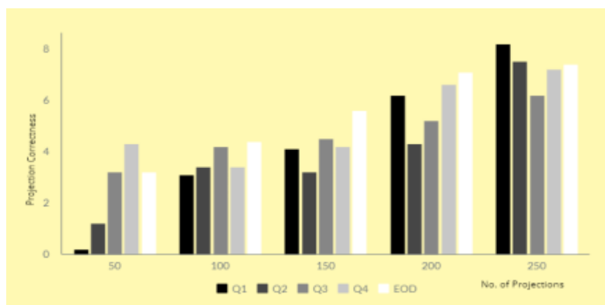
Projection Correctness
