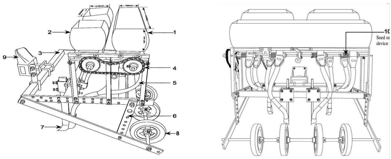
1. Seed box, 2. Fertilizer box, 3. Toolbar frame, 4. Chain and sprocket, 5. Seed tube, 6. A depth control device, 7. Furrow opener 8. Press wheel 9. Hitch plate 10. Seed metering device
